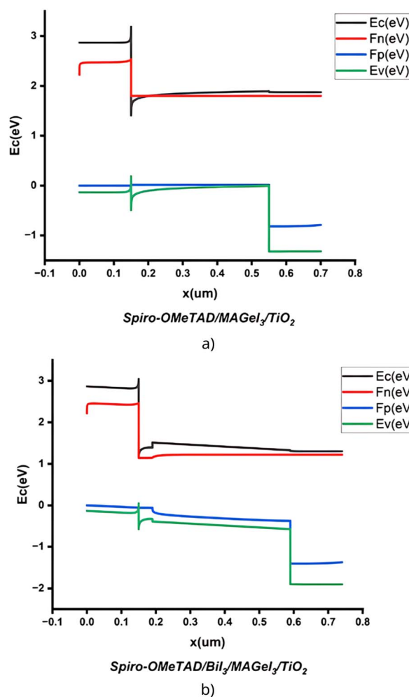
Fig. 13 Energy band alignment of the \text{MAGeI}_3 perovskite/HTL interface: (a) without and (b) with the \text{BiI}_3 interlayer. Reproduced and adapted from Noman et al. (2024) 75 (doi: https://doi.org/10.1038/s41598-024-56246-4 ) under a Creative Commons Attribution (CC BY 4.0) license.
