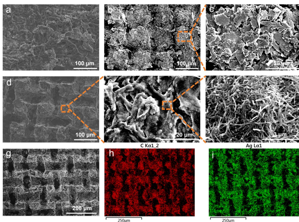
Fig. 2 The surface morphology of the T-eNFM printed electrode. (a) T-eNFM surface screen-printed conductive layer. (b) Microstructure of conductive layer of Ag paste printed on T-eNFM surface by screen printing and (c) its local magnified image. (d) Microstructure of conductive layer of MWCNTs and Ag paste printed on T-eNFM surface by screen printing and (e and f) local magnified image. (g) The surface screen printing of T-eNFM features a regular array of microstructure conductive layers and the distribution of (h) C element in the MWCNTs and (i) Ag element.
