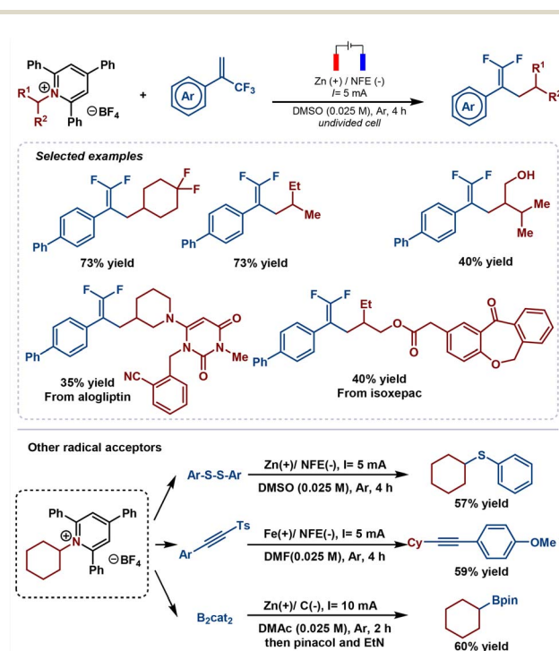
Scheme 19 Electrochemical deaminative functionalization of Katritzky salts with radical acceptors.
