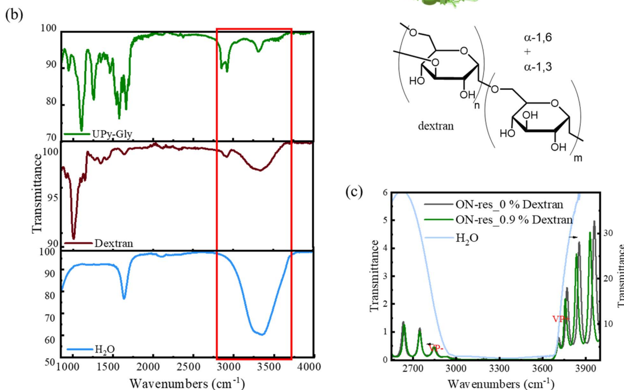
Fig. 2 (a) Molecular structure of UPy-Gly, UPy-Cy5 and dextran, and the schematic illustration of UPy-Gly and the corresponding supramolecular polymer. (b) FT-IR transmission spectra of UPy-Gly, dextran and water. The highlighted peaks represent the overlapping vibrational bands between the solutes and the solvent that are necessary for cooperative coupling. (c) FT-IR spectra showing the ON-resonance condition of the 1% UPy-Gly aqueous solution with and without dextran.
