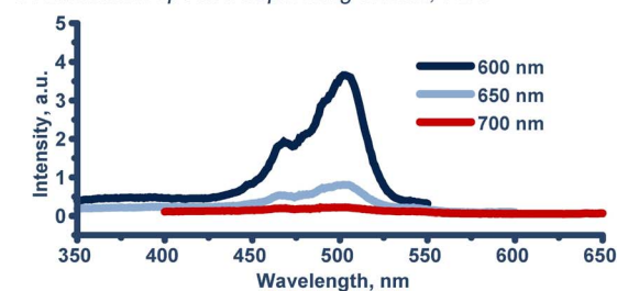
Fig. 4 Photophysical properties studies of 3. (A) Absorption spectra in acetonitrile as a function of percentage of water, 25 °C. (B) Emission spectra in PBS as a function of molarity of solution, RT. (C) Excitation spectra as a function of emission wavelength in PBS, RT (derived from Fig. S68–70†).
