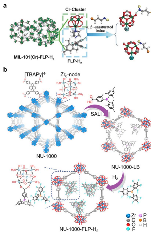
Fig. 13 (a) The "activation" process involving a \text{Cr}_3(\mu_3\text{-O})(\text{COO})_6(\text{OH})(\text{H}_2\text{O})_2 cluster in MIL-101(Cr)-FLP- \text{H}_2 . Reproduced with permission. 219 Copyright 2019, John Wiley and Sons. (b) Construction pathway of NU-1000-FLP- \text{H}_2 . Reproduced with permission. 220 Copyright 2023, American Chemical Society.
