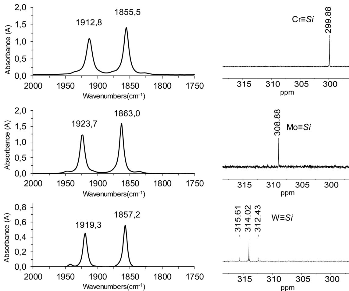
Fig. 5 (left) FT-IR spectra of the silyldiene complexes 1-Cr – 1-W in n -hexane in the spectral range 2000\text{--}1750\text{ cm}^{-1} showing the two \nu(\text{CO}) absorption bands; (right) ^{29}\text{Si}\{^1\text{H}\} NMR spectra (99.36 MHz) of 1-Cr – 1-W in ( D_6 )benzene at 298 K showing the \text{M}\equiv\text{Si} signals.
