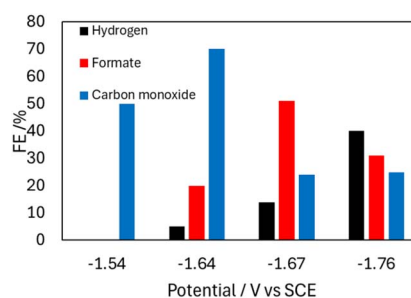
Fig. 6 Bar graph showing the product profile relative to E app , from CPE experiments performed with 0.1 mM 2 − in 0.1 M Bu 4 NBF 4 MeCN solution with 5 mM OMeBSulfH under 1 atm CO 2 over 20 min.
