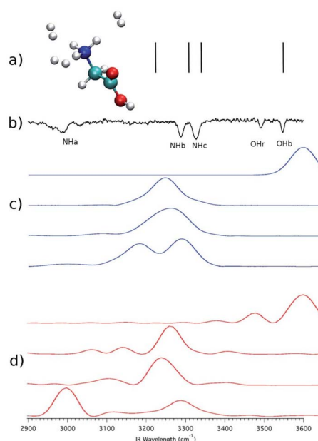
Fig. 1 Vibrational spectra for protonated glycine microsolvated by three H_2 molecules. Panel (a): harmonic estimates. Panel (b): the experimental spectrum; Panel (c): the quasi-classical trajectory method results; Panel (d): DC-SCIVR calculation. This figure has been reproduced from ref. 47 with permission from the Royal Society of Chemistry, copyright 2018.
