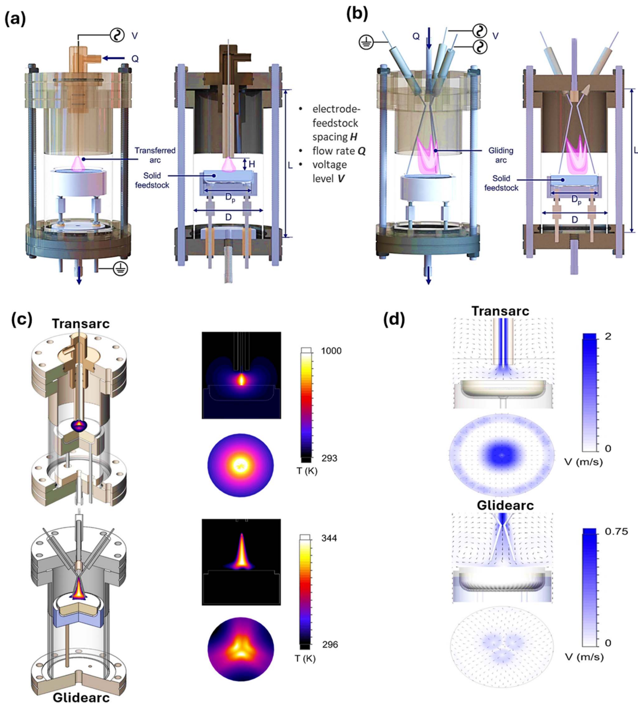
Fig. 10 Structural overview of (a) the transarc and (b) glidar arc low-temperature atmospheric pressure plasma reactors, (c) computational thermal fluid models for transarc and glidar arc reactors, along with the temperature distributions and (d) velocity distribution for the transarc and glidar arc reactors. Reproduced with permission from ref. 139. Copyright 2022, Elsevier.
