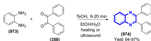
Scheme 270 Synthesis of 2,3-diphenyl quinoxaline catalyzed by PTSA.
