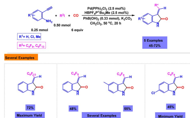
Scheme 22 Synthesis of fluorinated 3-methyleneoxindole derivatives through Pd(PPh₃)₂Cl₂ catalyzed one-pot three-component reactions of 2-ethynylanilines, per-fluoroalkyl iodides and carbon monoxide.
