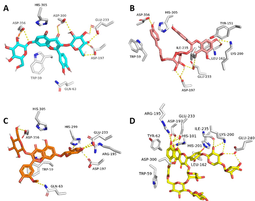
Fig. 5 Docking poses of compounds with docking scores < -10.0 \text{ kcal mol}^{-1} (i.e., 28, 61, and 64) along with the co-crystallized inhibitor montbretin A inside human \alpha -amylase ((A–D), respectively).
