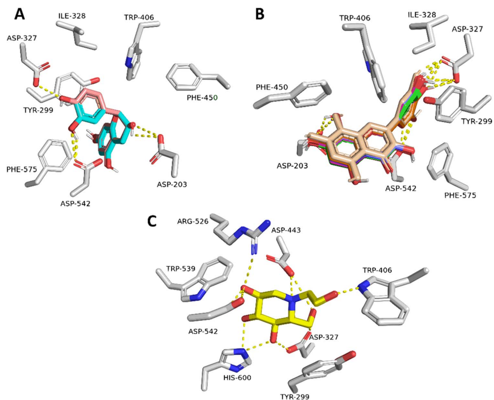
Fig. 6 Docking poses of compounds inside the human \alpha -glucosidase with docking scores < -10.0 \text{ kcal mol}^{-1} . (A) Compounds 10 and 39 (cyan and brick-red structures, respectively) aligned with each other. (B) Compounds 16, 17, 53, 69a, and 69b (green, blue, brown, pink, and orange structures, respectively) aligned with each other. (C) The co-crystallized inhibitor miglitol.
