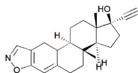
Danazole
