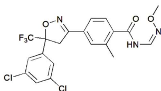
Fluxametamide
