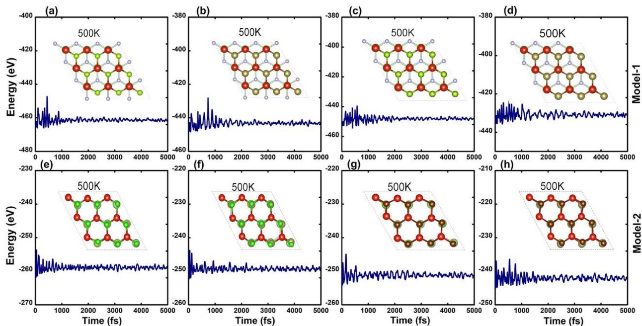
Fig. 2 AIMD simulations for model-I (a–d) and model-II (e–h) (GaN–VClSe, GaN–VClTe, GaN–VBrSe, GaN–VBrTe) at 500 K.
