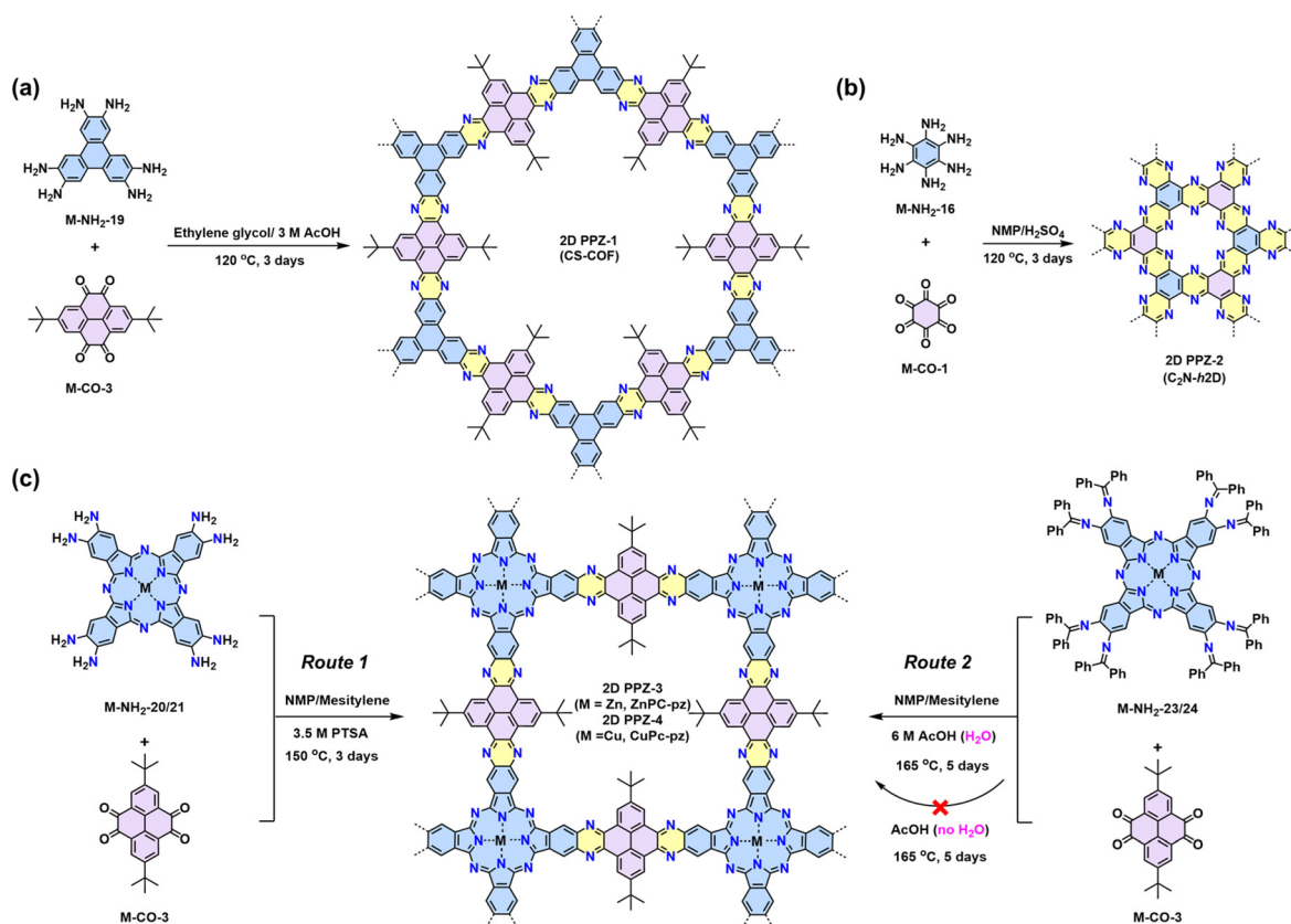
Scheme 2 (a) Synthesis of the first crystalline pyrazine-bridged 2D polypyrazine of 2D PPZ-1 (CS-COF). (b) Synthesis of 2D PPZ-2 crystals. (c) Two routes to synthesize 2D PPZ-3 ( ZnPC-pz ) and 2D PPZ-4 ( CuPC-pz ) with cubic lattice.
