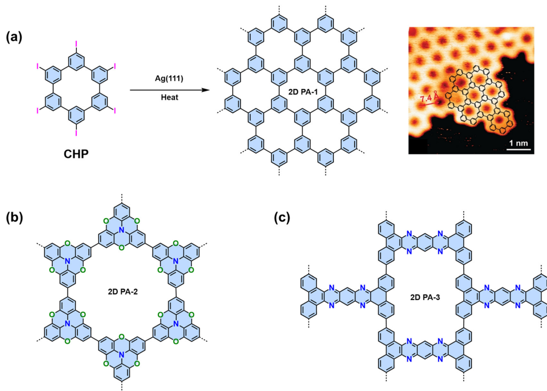
Fig. 7 (a) On-surface synthesis of 2D polyphenylene ( 2D PA-1 ) and the corresponding STM image. (b) Chemical structure of 2D PA-2 synthesized on Au(111) surface. (c) Chemical structure of 2D PA-3 synthesized by solid-state synthesis.
