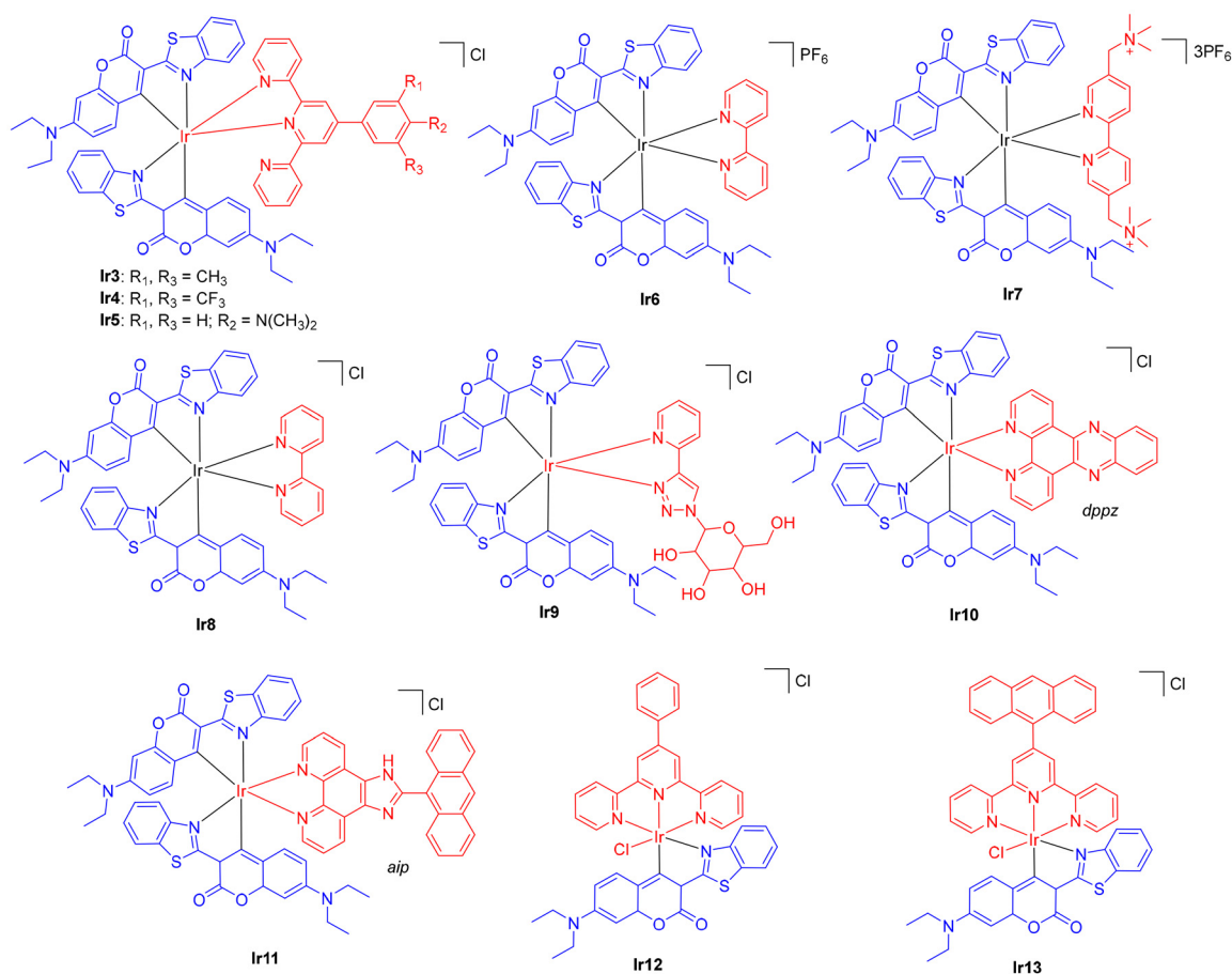
Fig. 9 Ir(III)-based PSs with coumarin C6 directly coordinated as C 6 N ligand.
