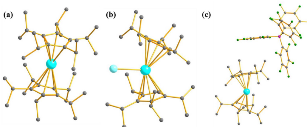
Fig. 15 The molecular structure of (a) [(\eta^5\text{-C}_5^i\text{Pr}_5)_2\text{U}]^+ ( 24 ) (b) [(\text{Cp}^i\text{Pr}_4)_2\text{U}] ( 25 ), and (c) [(\text{Cp}^i\text{Pr}_4)_2\text{U}][\text{B}(\text{C}_6\text{F}_5)_4] ( 26 ). Colour code: U (cyan), I (aqua), N (blue), Si (violet), B (pink), F (green), C (grey). Hydrogens are omitted for clarity.
