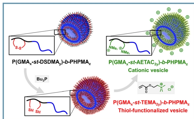
Fig. 3 Schematic illustration of surface-functionalized PISA vesicles based on disulfide cleavage of P(\text{GMA}_x\text{-st-DSDMA}_y)\text{-b-PHPMA}_2 . Adapted with permission from ref. 68. Copyright 2012 American Chemical Society.
