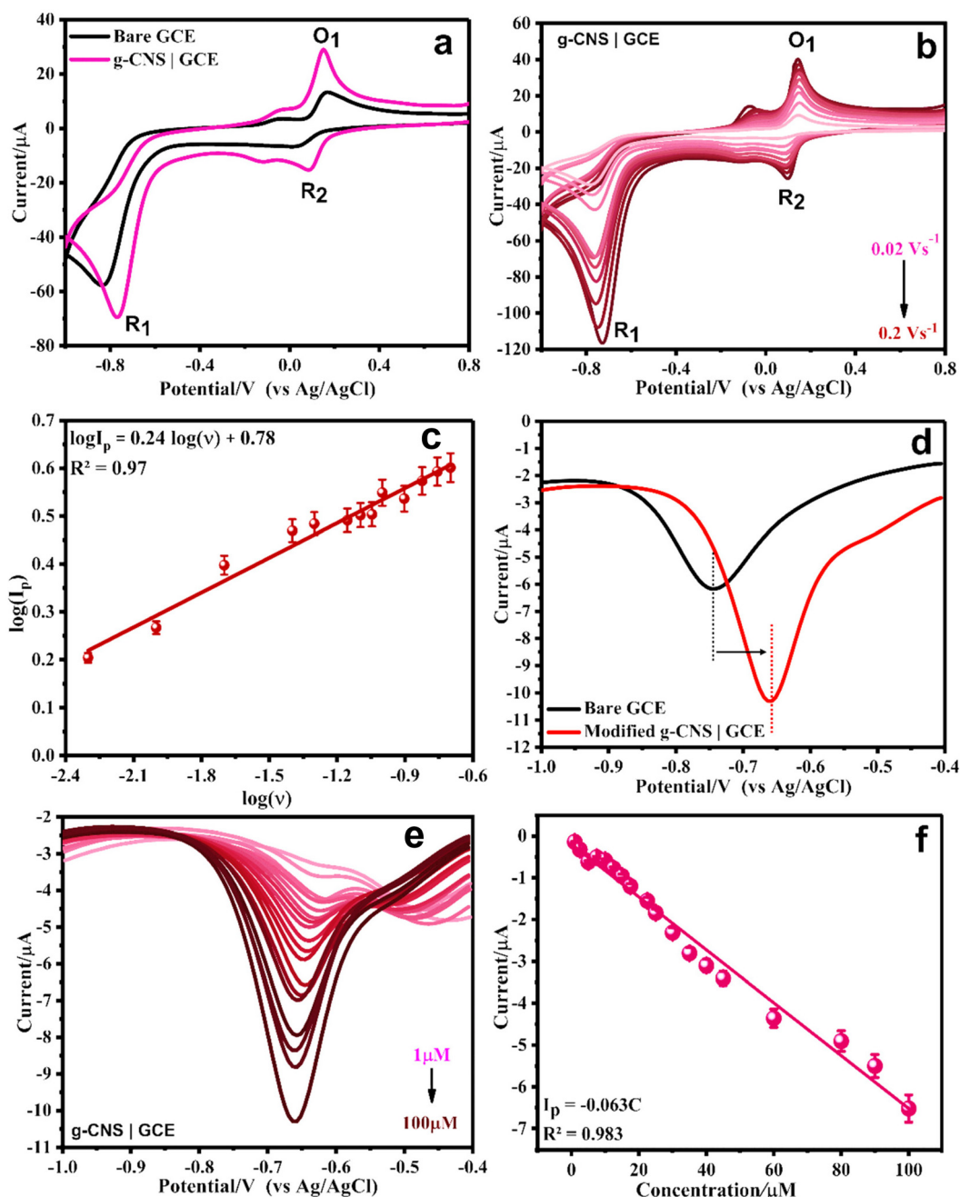
Fig. 5 (a) Comparative CV of 100 μM p -NP recorded using bare GCE and g-CNS|GCE. (b) CV of 100 μM p -NP as a function of varying scan rates ranging from 0.02 V s -1 to 0.2 V s -1 recorded using g-CNS|GCE. (c) Plot of log I p vs. log ν for the R 1 peak. (d) Comparative SWV graph of 100 μM p -NP recorded using bare GCE and g-CNS|GCE. (e) SWV peaks corresponding to increasing concentrations of p -NP ranging from 1 μM to 100 μM recorded using g-CNS|GCE. (f) Linear regression plot between peak current and concentration of p -NP. All the measurements were carried out using phosphate buffer of pH 7 as supporting electrolyte.
