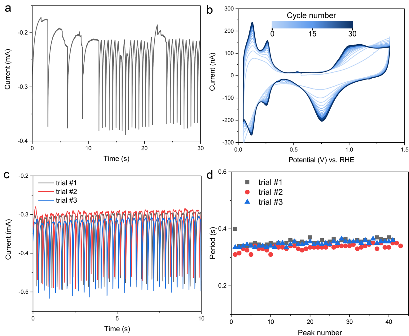
Fig. 2 This figure demonstrates the effect of the electrochemical pretreatment on reproducible electrochemical oscillation: (a) chronoamperometry curve of a 100\ \mu\text{m} Pt disk microelectrode without electrochemical pretreatment (measurement condition: 0.5\ \text{M}\ \text{H}_2\text{SO}_4 , -0.32\ \text{V}_{\text{RHE}} ). (b) Cyclic voltammogram during electrochemical pretreatment (pretreatment condition: potential cycling between 0.05 to 1.35\ \text{V}_{\text{RHE}} , 30 cycles at scan rate of 1\ \text{V}\ \text{s}^{-1} ). (c) Chronoamperometry curves after electrochemical pretreatment (measurement condition: 0.5\ \text{M}\ \text{H}_2\text{SO}_4 , -0.32\ \text{V}_{\text{RHE}} ). Each trial was performed on different days using the same electrode and procedure. (d) Period of electrochemical oscillation in (c).
