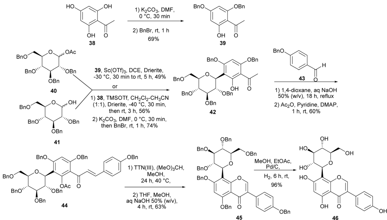
Scheme 6 Synthesis of 8- \beta -D-glucopyranosylgenistein (46).
