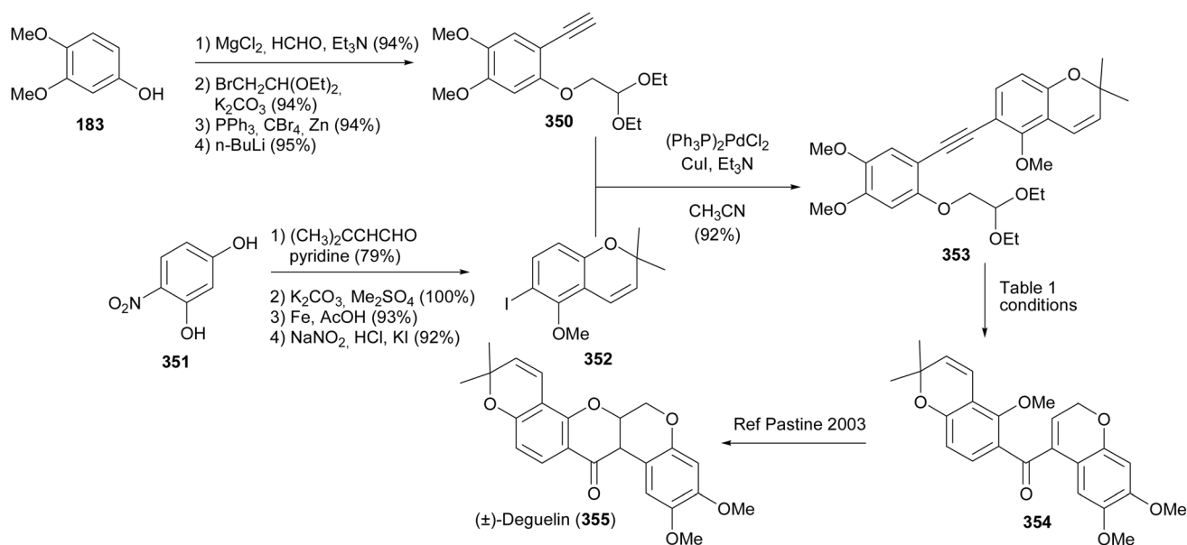
Scheme 49 Synthesis of (±)-deguelin (355).
