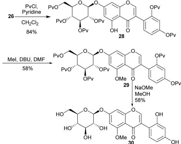
Scheme 4 Synthesis of isoflavone glucoside 30 .
