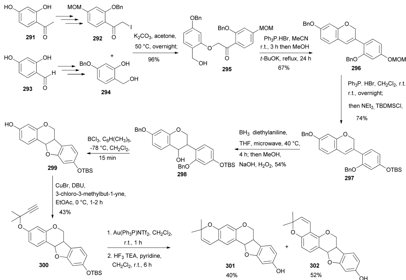
Scheme 43 Total syntheses of neorautenol (301) and shinpterocarpan (302).
