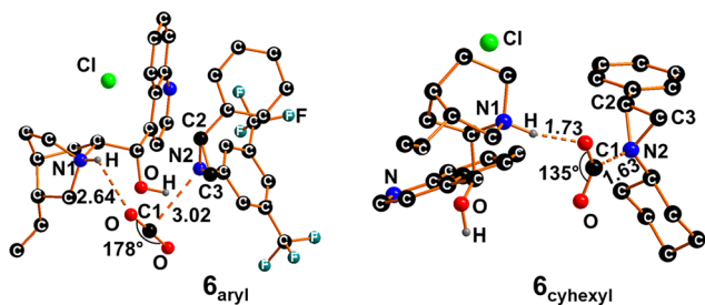
Fig. 6 Optimized structure of adducts \mathbf{6}_{\text{aryl}} and \mathbf{6}_{\text{cyclohexyl}} , presenting 1-(3,5-bis(trifluoromethyl)phenyl)-2-phenylaziridine and 1-cyclohexyl-2-phenylaziridine, respectively. The hydrogen atoms were hidden for the sake of clarity, except for those linked to a heteroatom. Selected distances are given in Å and O-C-O angle in degrees (°).
