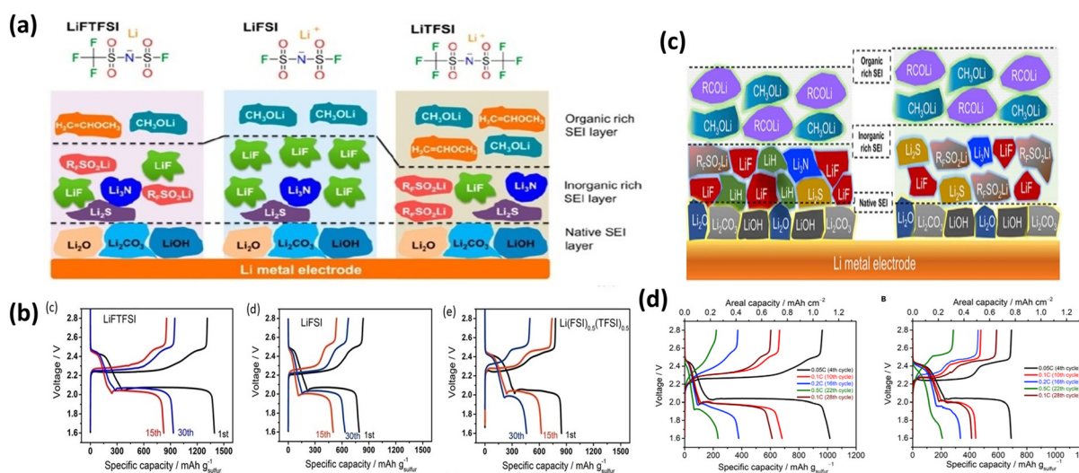
Fig. 10 Interaction of PEO with Li salts with different anions: (a) PEO–LiFTFSI, PEO–LiFSI and PEO–LiTFSI; (b) charge–discharge plots of salts in (a); (c) SEI layer formed on Li electrode with LiDFTFSI and LiTFSI salt; (d) charge–discharge plots of salts in (c). These figures have been reproduced from ref. 52 with permission from American Chemical Society copyright 2018 and from ref. 53 with permission Elsevier copyright 2019.
