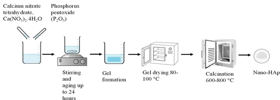
Fig. 4 Synthesis of hydroxyapatite by the sol-gel technique.
