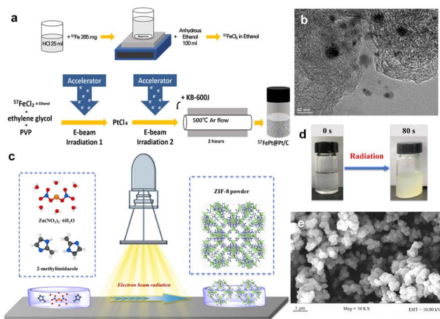
Fig. 4 (a) Schematic illustration of the synthesis of ^{57}\text{FePt}@\text{Pt}/\text{C} via electron-beam irradiation. (b) TEM image of ^{57}\text{FePt}@\text{Pt}/\text{C} . Copyright 2023 Wiley-VCH. (c) The synthesis setup of ZIF-8 via electron beam radiation. (d) The photo of ZIF-8 synthesized at an absorbed dose of 50 kGy. (e) SEM image of ZIF-8 at an absorbed dose of 50 kGy. 54,55 Copyright 2022, Wiley-VCH.
