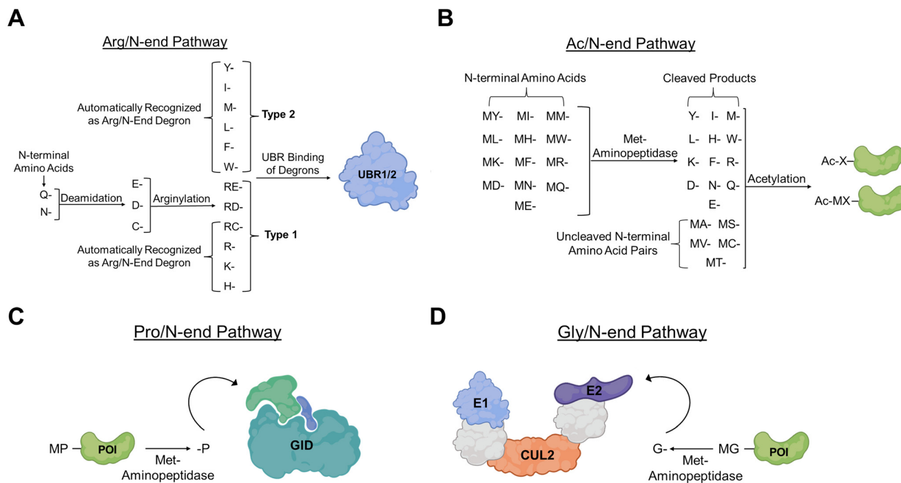
Fig. 3 N-degion pathways. (A) Arg/N-end degion pathway. UBR1/2 serves as the main E3 ligase for substrate recognition of Arg/N-end degrons. N-terminal proteins are recognized at three stages: tertiary (Q, N), secondary (C, D, E), and primary (R, K, H, W, L, F, Y, I). Tertiary amino acids are converted to secondary via the conversion of their amide substituent to a carboxylic acid. Secondary amino acids are converted to primary via conjugation to the amino acid Arg. The final primary substrates are recognized by two distinct substrate binding sites of UBR, one binding positively charged residues (type 1) and the other binding bulky hydrophobic residues (type 2). (B) Ac/N-end degion pathway. N-terminal acetylated proteins can serve as degrons for many protein substrates. Many N-terminal degrons that are acetylated are recognized at either N-terminal Met or N-terminal Met pairs (MA, MS, MV, MC, MT). Unpaired Met are cleaved via Met-aminopeptidases and both degrons are subsequently acetylated and degraded. (C) Pro/N-end degion pathway. Met cleavage can lead to recognition of N-terminal Pro residues by the GID E3 ligase complex. (D) Gly/N-end degion pathway. Met cleavage also can result in the recognition of N-terminal Gly residues by the Cul2 E3 ligase complex.
