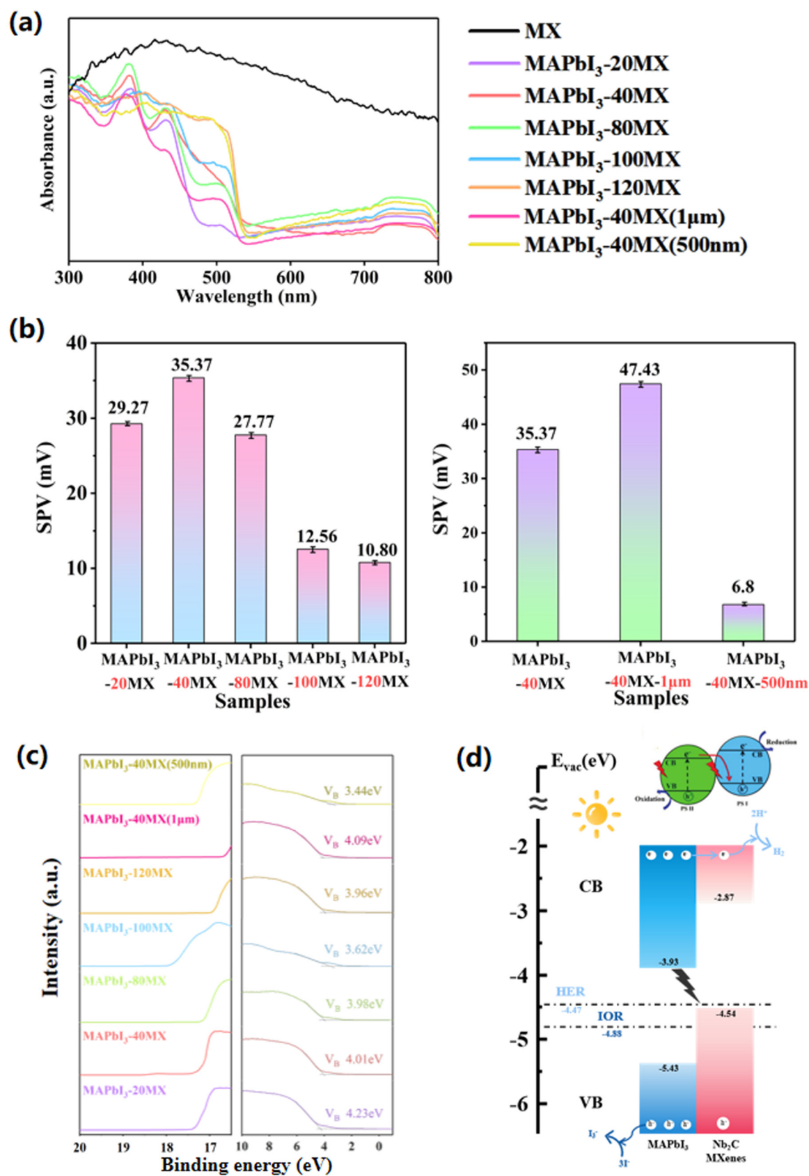
Fig. 4 (a) UV-vis spectra and band gap energies of composite Nb 2 CT x MXenes and MAPbI 3 at different ratios. (b) SPV signals of composite Nb 2 CT x MXenes and MAPbI 3 at different ratios. (c) UPS spectra of composite Nb 2 CT x MXenes and MAPbI 3 at different ratios. (d) Schematic band diagram of MAPbI 3 /Nb 2 CT x MXenes for photocatalytic H 2 splitting reactions.
