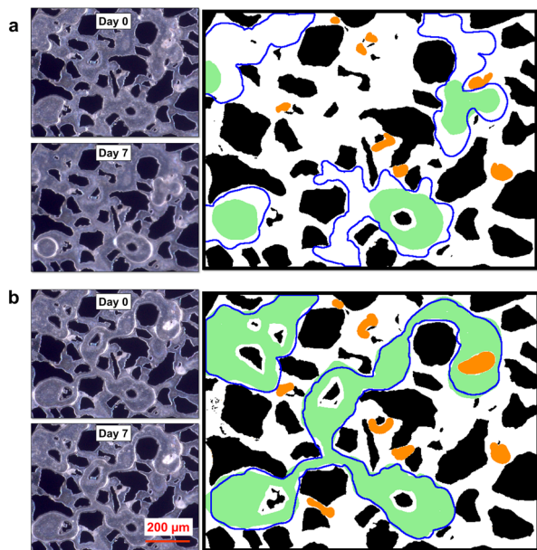
Fig. 4 Bio-geochemical interactions during porous media hydrogen storage. (a) Microbial hydrogen consumption in a calcite-functionalized micromodel: inoculated microbial cells utilized hydrogen gas as an electron source for sulfate reduction. Over the seven-day experiment, continuous microbial activity led to hydrogen gas consumption, with no observed changes in CaCO 3 precipitation. (b) Interaction of calcite with pure hydrogen gas without microbes: the interaction between hydrogen gas and calcite was studied under pressures ranging from 10 to 100 barg. Under these conditions, both the gas and calcite remained unchanged over time. The left column shows original microscopy images, whereas the right column presents conceptual representations (blue outlines: gas distribution at day 0; green: gas distribution at day 7, orange: calcite precipitates; black: grains; white: aqueous phase). Experimental conditions were P = 30 barg, T = 37.5 \pm 0.5 °C. Details of the experimental procedure are provided in the ESI.†
