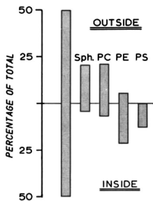
Fig. 1 From Verkleij et al. 1973 (ref. 13) originally BBA, 323 : 190 Fig. 13. Note that error bars, which are likely significant, are not available.
