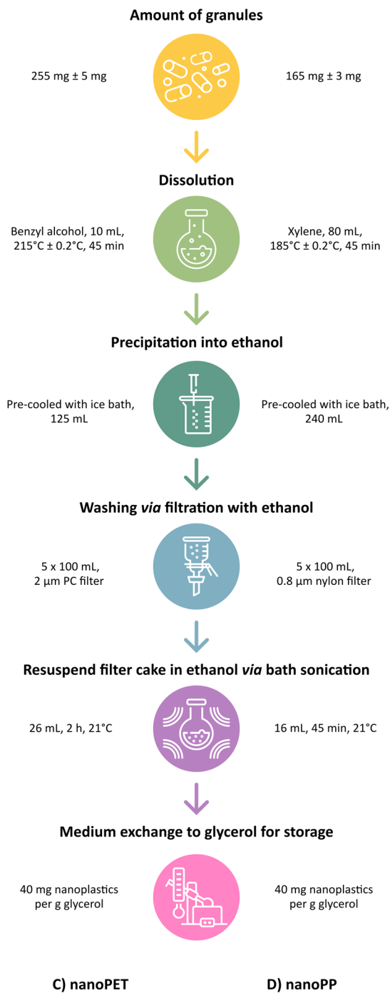
Fig. 2 Production scheme of PET (A) and PP (B) nanoplastic suspensions. Overview of controlled parameters and the experimental settings used. Representative SEM micrographs of PET (C) and PP (D) nanoplastics.
