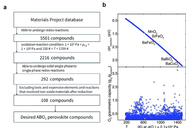
Fig. 2 (a) Screening workflow by Lau et al. , 67 plotted based on the description in the manuscript and SI data; (b) overview of the key results from screening the Materials Project database for compounds that undergo redox reactions. 67 The predicted reduction temperature at P_{O_2} = 2.1 \times 10^4 Pa for each reaction is plotted against \Delta H_{\text{reduction}} (upper panel) and O_2 gravimetric capacity (lower panel). (b) is adapted from ref. 67 with permission from the Royal Society of Chemistry, copyright 2017.
