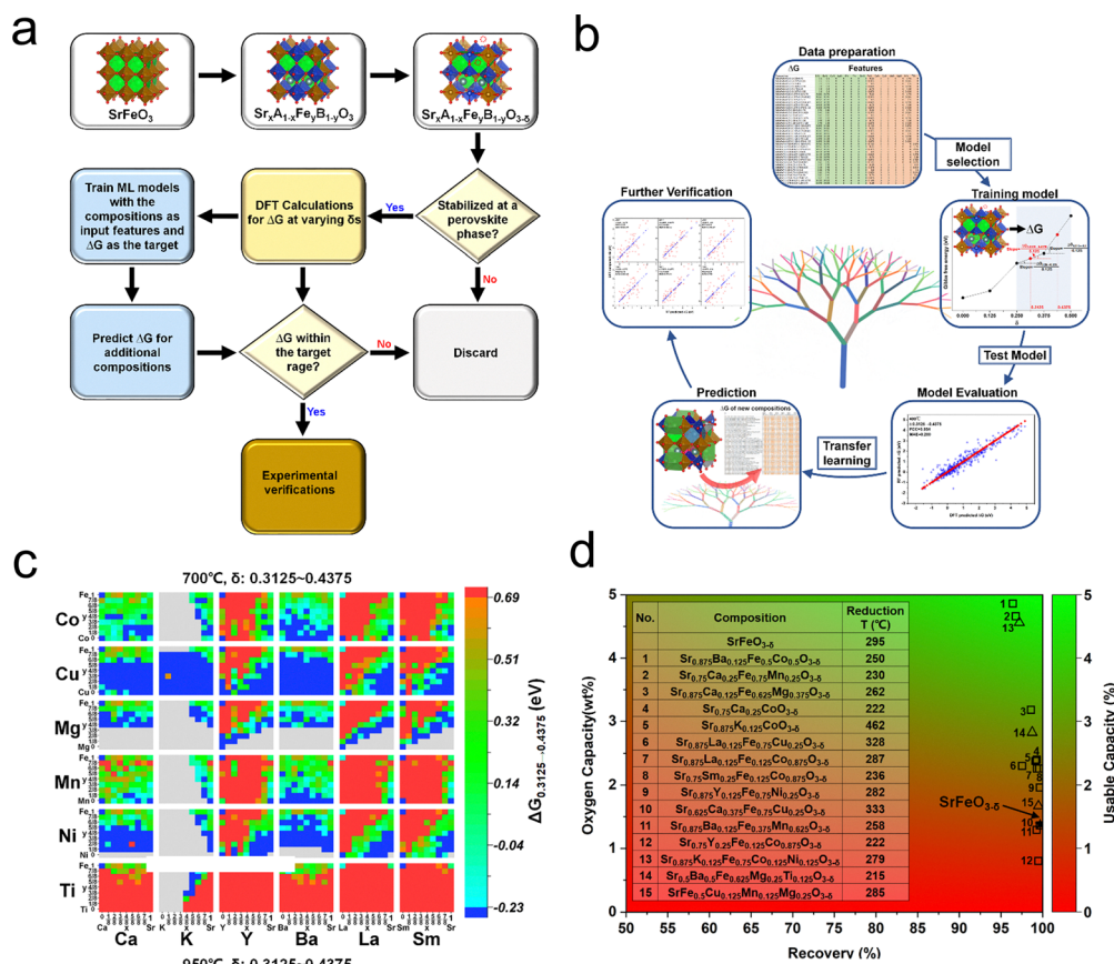
Fig. 3 (a) DFT model construction, high-throughput calculations, and materials screening. (b) ML steps for the training, evaluation, and prediction of perovskite datasets. Heatmap of the screened candidates for (c) CLAS at 700 °C within the \delta range of 0.3125–0.4375. (d) Experimental oxygen capacity, recovery, and usable capacity of the samples tested for CLAS. Squares and circles represent DFT- and ML-predicted samples, respectively. 74 This figure is adapted from ref. 74 with permission from the Royal Society of Chemistry, copyright 2021.
