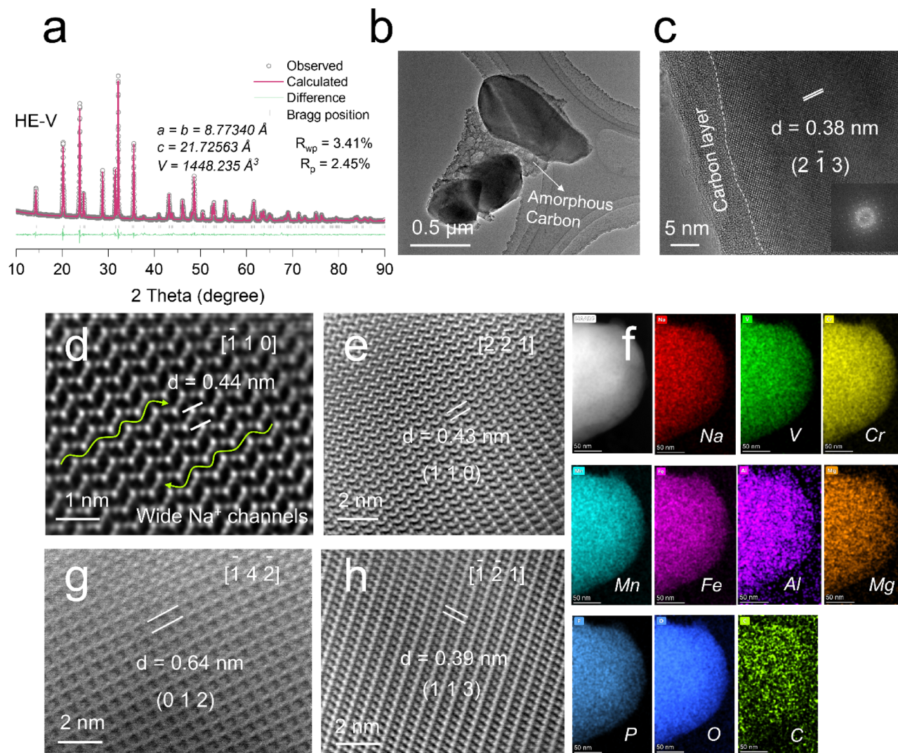
Fig. 2 Material characterization of HE-V. (a) XRD Rietveld refinement results. (b) and (c) TEM and HRTEM images. (d)–(h) Aberration-corrected STEM images viewed from the (d) [1\bar{1}0] , (e) [221] , (g) [14\bar{2}] , and (h) [1\bar{2}1] crystallographic directions. (f) EDS mapping images (scale bar: 50 nm).
