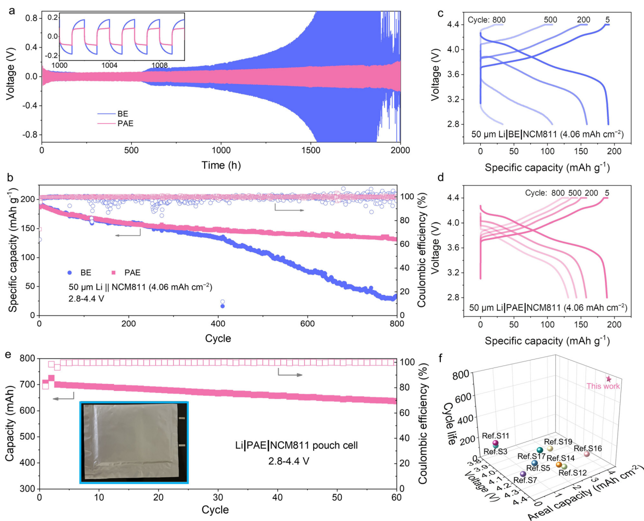
Fig. 6 Practical electrochemical performances. (a) Cycling performance of symmetric LMBs with various electrolytes at a current density of 0.5 mA cm -2 (0.5 mA h cm -2 ). The inset provides a detailed view from the 1000th to the 1010th cycle. (b) Cycling performance of 50 μm Li||NCM811 (4.06 mA h cm -2 ) cells with various electrolytes cycled at 0.2C charge and 0.3C discharge (1C = 200 mA g -1 ). (c) Charge-discharge voltage profiles of the 50 μm Li||NCM811 (4.06 mA h cm -2 ) cell using BE. (d) Charge-discharge voltage profiles of the 50 μm Li||NCM811 (4.06 mA h cm -2 ) cell using PAE. (e) Cycling performance of the Li||NCM811 (692 mA h) pouch cell with an energy density of 397 W h kg -1 (inset: the digital photo of the pouch cell; 0.2C charge/0.3C discharge). (f) Performance comparison of the cell with PAE against published studies involving SPEs (more data are detailed in Table S5, ESI†).
