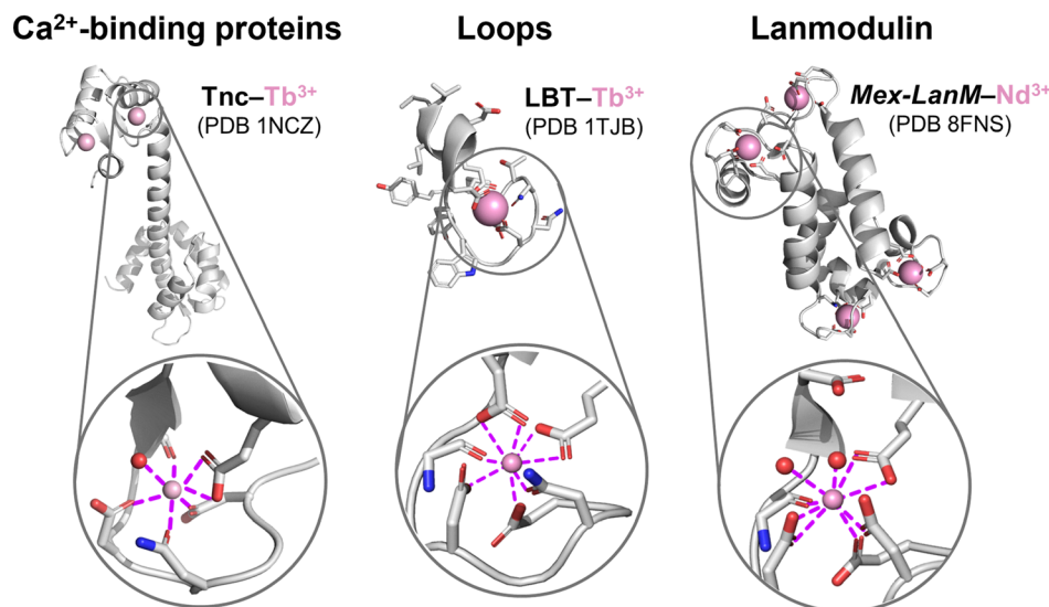
Fig. 4 EF-hand peptides and proteins. Top: EF-loop sequence showing the most common Ln 3+ -binding amino acids (in bold and highlighted in pink) in each position. Bottom: Protein structures and Ln 3+ coordination spheres in: left, troponin C (TnC) bound to two Tb 3+ ions (PDB 1NCZ); middle, a lanthanide-binding tag (LBT) bound to Tb 3+ (PDB 1TJB); right, Mex-LanM bound to four Nd 3+ ions (PDB 8FNS). Figures were generated using Pymol.
