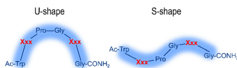
Fig. 5 Schematic structures of short cyclic (A) and linear (B) Ln-binding peptides. In (B) the structures of unnatural amino acids Xxx = Ada n and Ed3a 2 , and shapes adopted by linear peptides are shown. Adapted from ref. 8.
