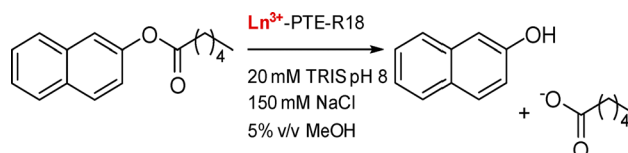
Fig. 29 Hydrolysis of 2-naphthyl hexanoate by Ln-PTE-R18.
