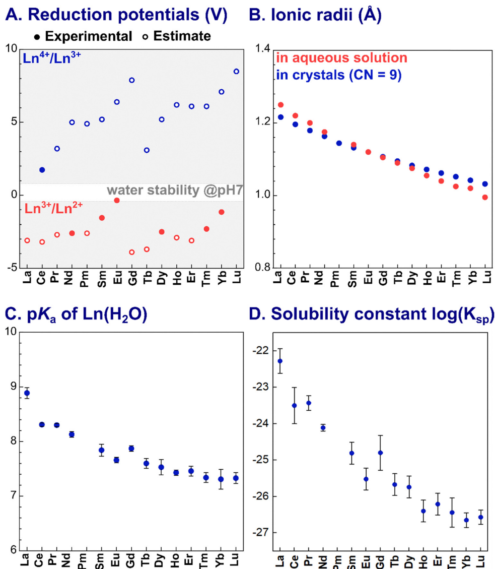
Fig. 1 Trends of key parameters along the Ln series: (A) reduction potentials; 26 (B) ionic radii in aqueous solution 27 and in crystals (CN = 9); 28 (C) acidity constants ( pK_a ) for \text{Ln}^{3+} -bound water molecule; and (D) solubility constants ( \log K_{sp} ). 29 The values plotted are reported in Table 14.
