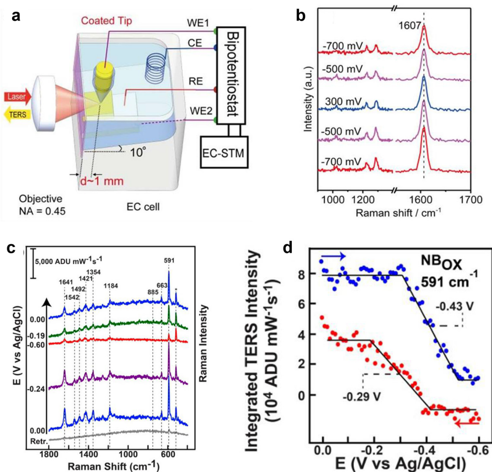
Fig. 39 The electrochemical TERS (EC-TERS). (a) The schematics of EC-TERS setup. (b) The potential dependent EC-TERS spectra of 4-PBT adsorbed on Au(111) surface. Tip potential was -200 \text{ mV} , and the tunneling current was 500 \text{ pA} . (c) EC-TES spectra of NB acquired at different potentials during cyclic voltammetry showing reversible reduction and oxidation of NB. P = 110 \text{ }\mu\text{W} , t = 1 \text{ s} , \lambda = 633 \text{ nm} , scan rate = 10 \text{ mV s}^{-1} . The asterisk denotes the Si Raman band from the AFM tip. (d) Potential dependence of the integrated TERS intensity of the 591 \text{ cm}^{-1} band of \text{NB}_{\text{ox}} . Figures are reproduced from ref. 371 and 372 with permissions. Copyright 2015 American Chemical Society.
