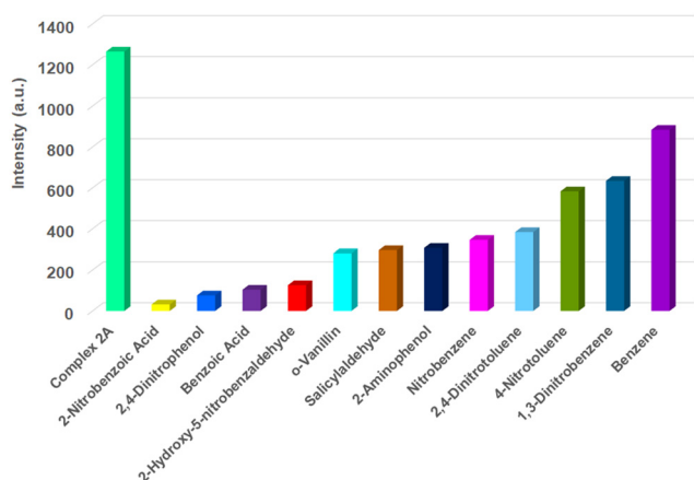
Fig. 14 Relative fluorescence intensity change profile of complex 2A in the presence and absence of various aromatic quenchers ( 10^{-2} \text{ M} ) at room temperature (excitation at 379 nm).
