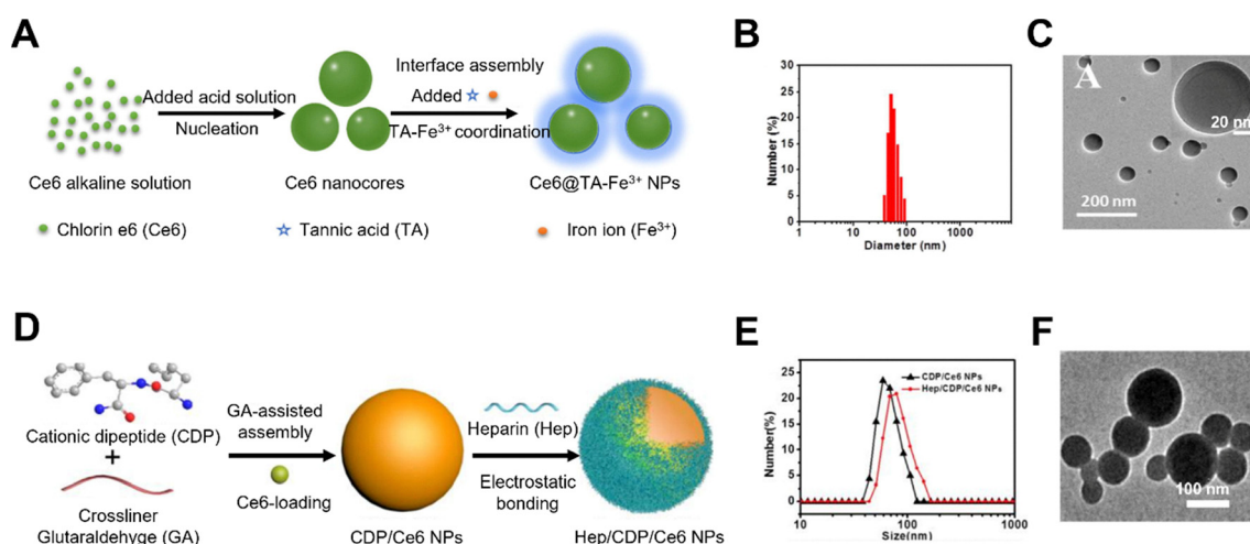
Fig. 3 Assembly strategy. (A) Interface-directed assembly of Ce6-encapsulated \text{TA-Fe}^{3+} nanoparticles. (B) DLS result and (C) TEM image of \text{Ce6@TA-Fe}^{3+} NPs. Adapted from ref. 28, with permission from 2017, The Author(s). (D) Covalent crosslinked assembly of dipeptides and glutaraldehyde, with Ce6 encapsulation and heparin surface modification. (E) DLS result and (F) TEM image of Hep/CDP/Ce6 NPs. Adapted from ref. 31, with permission from 2016, American Chemical Society.
