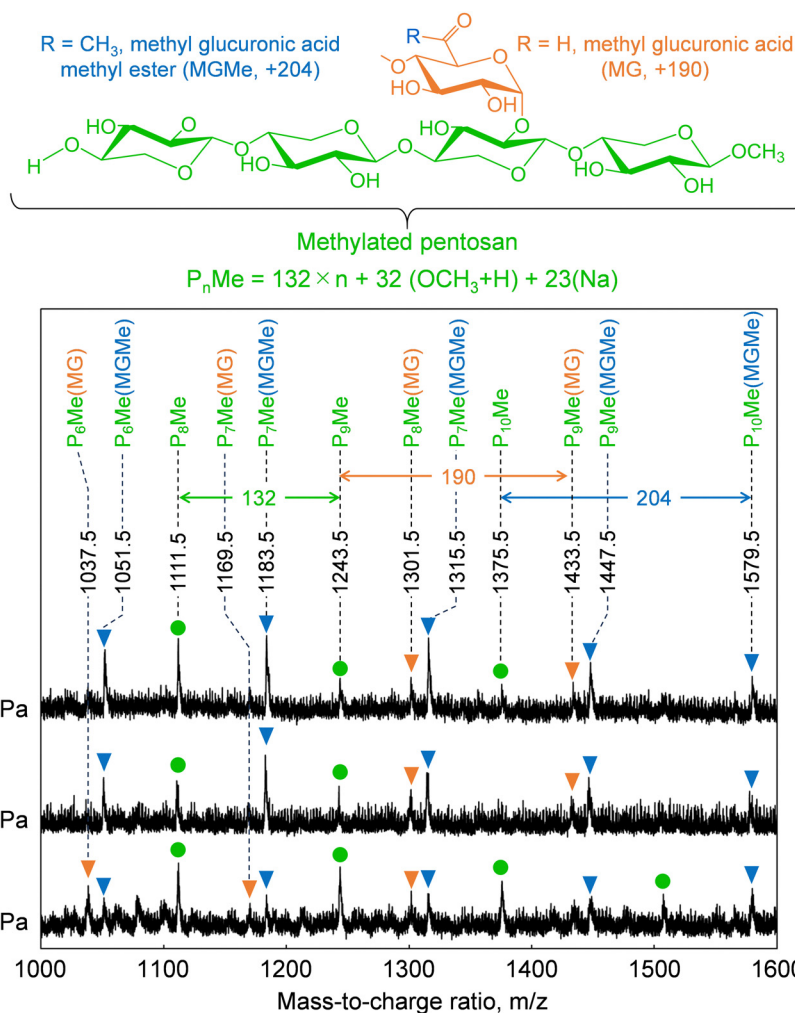
Fig. 8 Matrix-assisted laser desorption ionization-time-of-flight mass spectra of oligosaccharides obtained from holocellulose after treatment with methanol/water (90/10, v/v) at various pressures.
