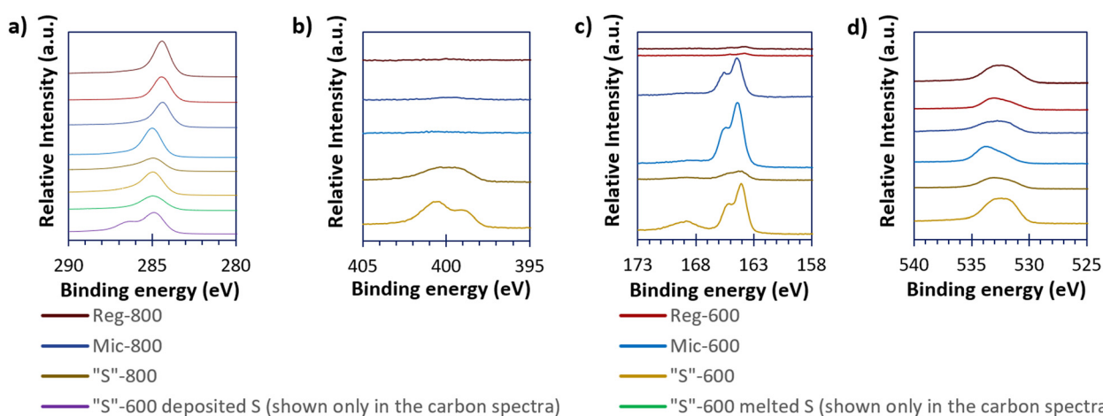
Fig. 5 The high resolution XPS spectra of the carbonaceous (and the "S"-600/S composites) materials of C 1s (a), N 1s (b), S 2p (c), and O 1s (d).
