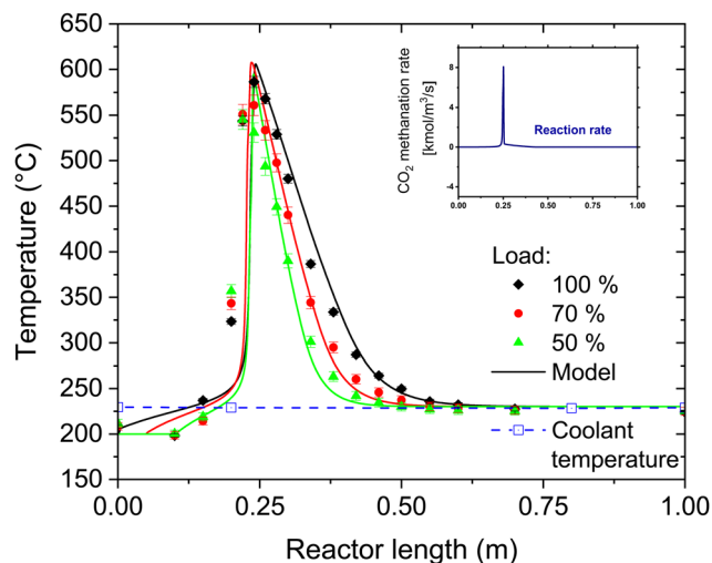
Fig. 5 Temperature profile at different load cases and modelling results (experimental conditions: 8 bar, H_2 : CO_2 = 4.15 , CO_2 : CH_4 = 1 : 1 , cooling setpoint = 230 °C, biogas flow = 22 N m 3 h -1 , 80 kg of catalyst in the reactor). The error bars refer to the variation of the temperature in the various experimental runs. In the insert, the calculated methane formation rate (mol L -1 s -1 ) is displayed. The temperature of the coolant remained constant over the entire reactor throughout the experimental tests.
