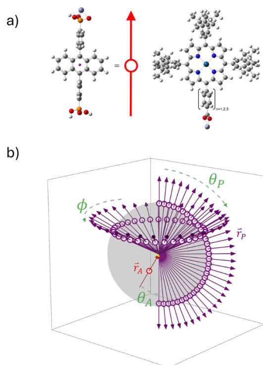
Fig. 7 a) Vector representations of the transition dipole moments of A (red) and PX (purple) with the chromophore centroid depicted as a circle. (b) Geometric orientation of vectors showing permutation by altitudinal ( \theta_P ) and azimuthal ( \phi ) rotation. In this model space, \theta_P is defined as the angle to the positive z-axis and \phi is defined as the angle between the projection of r_P onto the x,y-plane and the positive x-axis
