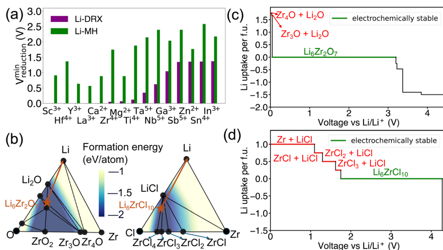
Fig. 3 (a) The minimum cathodic limits (referenced to \text{Li}/\text{Li}^+ ) for Li reduction of Li-DRX and Li-halide and (b) phase diagram of Li-Zr-O and Li-Zr-Cl. The formation energy of compositions in the convex hull is illustrated by the color contour, the stable phases are shown by black circles, the target compounds are marked as orange stars and orange arrows illustrate the decomposition pathways of \text{Li}_6\text{Zr}_2\text{O}_7 and \text{Li}_6\text{ZrCl}_{10} , respectively. The equilibrium voltage profiles and phase equilibria for lithiation reactions of (c) \text{Li}_6\text{Zr}_2\text{O}_7 and (d) \text{Li}_6\text{ZrCl}_{10} . The decomposition products of lithiation reactions at the anode side are labeled in red color, and the electrochemically stable voltage range is marked in green color.
