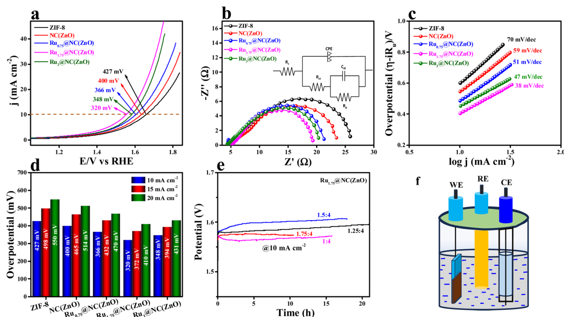
Fig. 3 (a) LSV polarization results of ZIF-8, NC(ZnO), Ru_{0.75}@NC(ZnO) , Ru_{1.75}@NC(ZnO) and Ru_3@NC(ZnO) ; (b) EIS outcomes; the inset shows the equivalent circuit diagram; (c) iR drop free Tafel slope; (d) overpotential measured at different current densities; (e) long term-static stability at an applied current density of 10\text{ mA cm}^{-2} ; (f) cell representation of the three-electrode setup used for OER performance.
