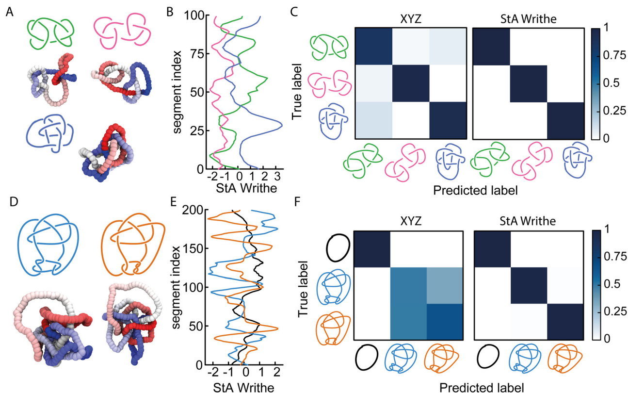
Fig. 2 (A) Snapshots of three knots with identical Alexander polynomial: square ( 3_1^2\#3_1^2 ), granny ( 3_1^2\#3_1^2 ) and 8_{20} knots. (B) Examples of StA writhe patterns from the three knots. (C) Confusion matrices obtained from a 3-class classification problem, training a FFNN with XYZ (91.7% accuracy) or StA writhe (99.9% accuracy) features. (D) Snapshots of Conway (blue) and KT (orange) knots. (E) Examples of StA writhe patterns, including the one from the unknot (black). (F) Confusion matrices obtained from a 3-class classification problem, training a FFNN with XYZ (67% accuracy) and StA writhe (99.6% accuracy).
