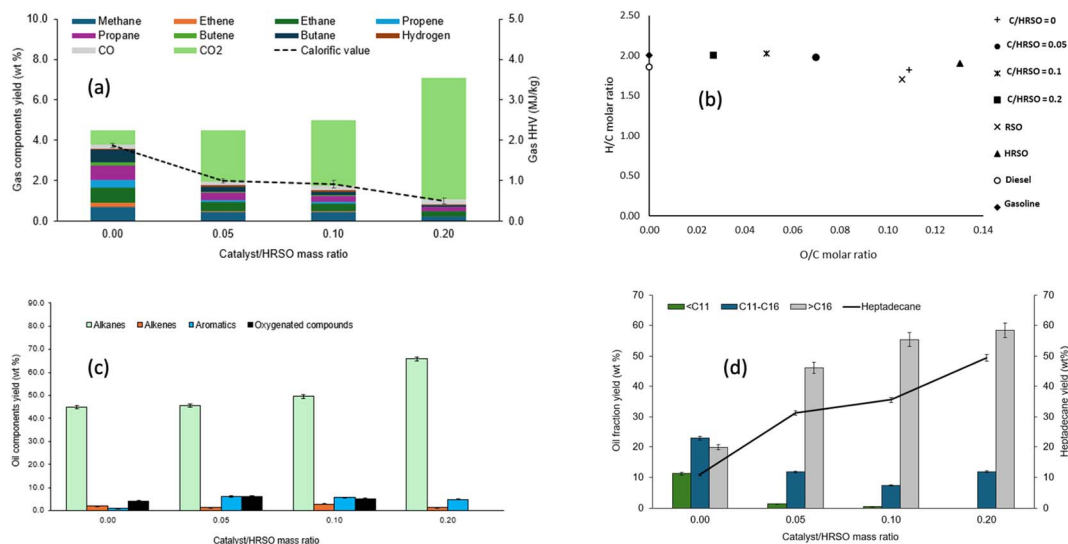
Fig. 4 Influence of 5 wt% Pt/C catalyst/HSRO mass ratios on (a) the compositions and calorific values of gas products, (b) the van Krevelen H/C and O/C molar ratios of the oil products, (c) the yields of groups of compounds in the light oils and (d) the yields of hydrocarbons and heptadecane in the light oil.
