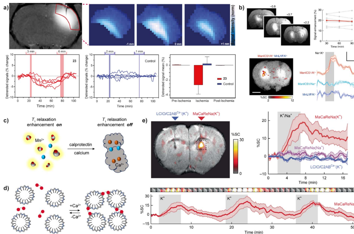
Fig. 4 Calcium-responsive probes (second part). Functional MRI experiments in vivo with \text{Ca}(\text{II}) -sensitive CAs. (a) MRI images of probe 23 in the rat somatosensory cortex (upper left) and the regions of interest (ROIs) with signals enhanced by a paramagnetic probe <math><3\text{ mm}</math> away were recorded and analyzed (upper right), while transient cerebral ischemia was induced via occlusion of the middle cerebral artery. The collected signals showed significant signal fluctuations using probe 23 (lower left) compared to the control probe that is \text{Ca}(\text{II}) -insensitive (lower middle) during the pre-ischemia, ischemia, post-ischemia periods. Average values of the detrended signals indicate that only 23 can detect changes in the \text{Ca}(\text{II}) concentration (lower right). (b) The use of probe 24 to detect neural activation in rat brain. Infusion of 24 or the control agent (left and right, respectively) into the rat striatum resulted in the signal enhancement (upper left), with an average MRI signal increase by 20 \pm 2\% (upper right); under \text{K}^+ stimulation, only the brain area perfused with probe 24 showed an increase in MRI signal (lower left). The time course of mean MR signals exhibited significantly greater changes during \text{K}^+ stimulation with probe 24 then both control experiments using \text{Na}^+ stimulation with probe 24 or \text{K}^+ stimulation with the control probe (lower right). (c) Mechanism of \text{Ca}(\text{II}) -triggered T_1 -weighted MRI change of the NP-calprotectin; in the presence of \text{Ca}(\text{II}) , NP-calprotectin prevents the contact between free paramagnetic \text{Mn}(\text{II}) and water, reducing MRI signals. (d) Mechanism of \text{Ca}(\text{II}) -triggered T_2 -weighted MRI change of the probe NP-MaCaReNa. In the presence of \text{Ca}(\text{II}) , the C2AB moieties (red) induce the aggregation of nanoparticles prepared by coating oleate-stabilized magnetic iron oxide cores with a mixture of PC and PS (grain), changing MRI signals. (e) MRI experiments with NP-MaCaReNa in living rat brain. MRI signal increases in the presence of NP-MaCaReNa but not controls (right and left, respectively) (upper left). The time courses of MR signals near areas of contrast-agent delivery show that \text{K}^+ infusion (grey shading) in the presence of NP-MaCaReNa induces clear responses (red trace), whereas controls barely affect the MRI signal (upper right). The average time courses of three consecutive \text{K}^+ stimuli (grey shading) show the reproducibility of NP-MaCaReNa responses (bottom). Adapted with permission from: (a) ref. 53 Copyright © 2019 National Academy of Sciences, (b) ref. 59 Copyright © 2019, The Author(s), (e) ref. 63 Copyright © 2018, The Author(s).
