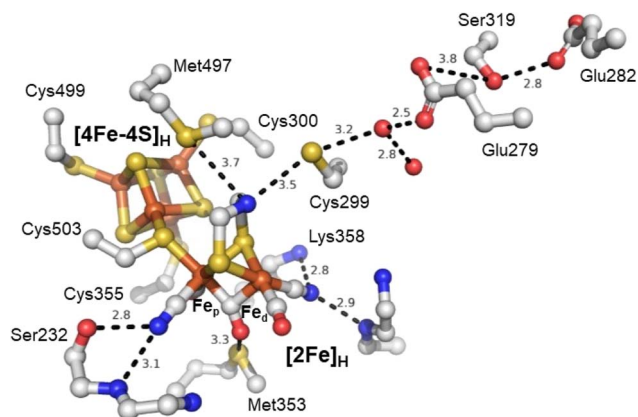
Fig. 4 Structure of the active site H-cluster of [FeFe] hydrogenase showing the interacting amino acid residues and proton transfer pathway. Distances shown are in Å. Residue numbering is from the C. pasteurianum enzyme. The image was prepared using PDB ID 4XDC. 24
