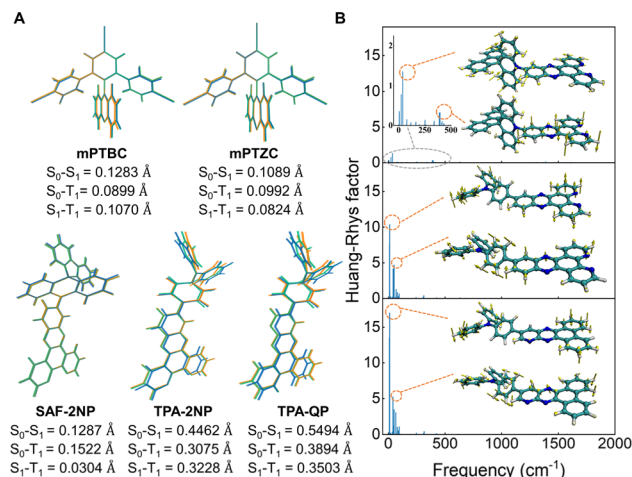
Fig. 2 (A) S 0 , S 1 and T 1 (in blue, orange and green, respectively) geometry variations of the five monomers and the corresponding RMSD values. (B) Calculated S 0 - S 1 Huang-Rhys factors of SAF-2NP (upper), TPA-2NP (middle) and TPA-QP (lower) at different frequencies (inset: representative vibrational modes).
