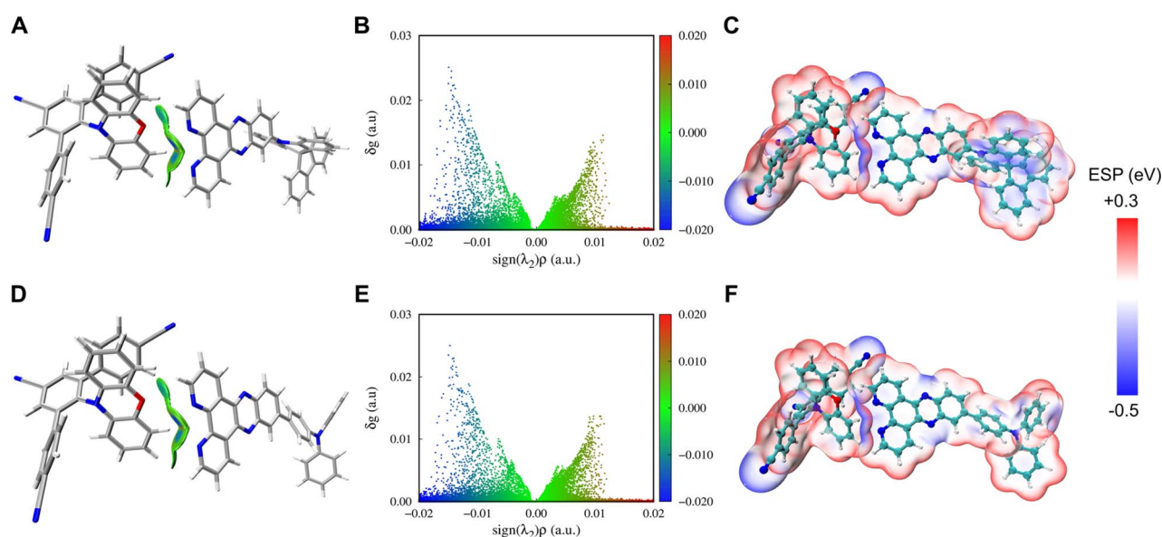
Fig. 3 Isosurface maps of intermolecular interaction based on optimized geometry (isoval = 0.003 a.u., color range: \pm 0.02 a.u.), corresponding scatter plots and ESP maps of mPTBC : SAF-2NP (A–C) and mPTBC : TPA-2NP (D–F).
