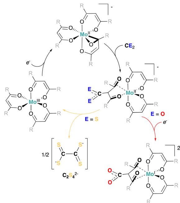
Scheme 3 Generalized mechanistic pattern for the reactivity of [\text{Mo}^{\text{R}}(\text{diket})_3]^{-1} with \text{CO}_2 (red arrow) vs. \text{CS}_2 (yellow arrow).
