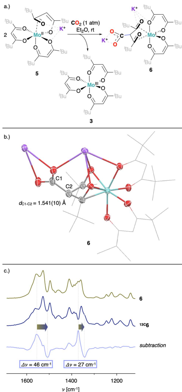
Fig. 6 (a) Reaction of 5 upon exposure to \text{CO}_2 . (b) XRD solid state structure of 6 . (c) IR-spectrum of 6 (green), ^{13}\text{C}\textbf{6} (dark blue) and the corresponding subtraction spectrum (light blue).
