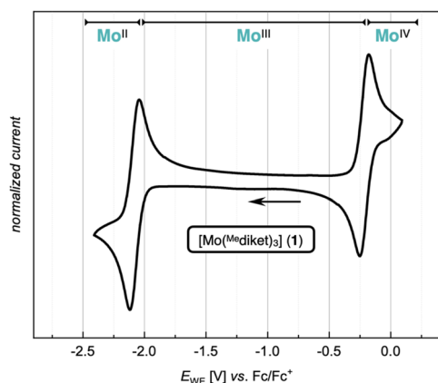
Fig. 2 CV of [\text{Mo}^{\text{IV}}(\text{Me}^2\text{diket})_3] ( 1 ) (1 mM) in \text{TBAPF}_6/\text{MeCN} (0.1 M) at a scan rate of \nu = 100 \text{ mV s}^{-1} .
